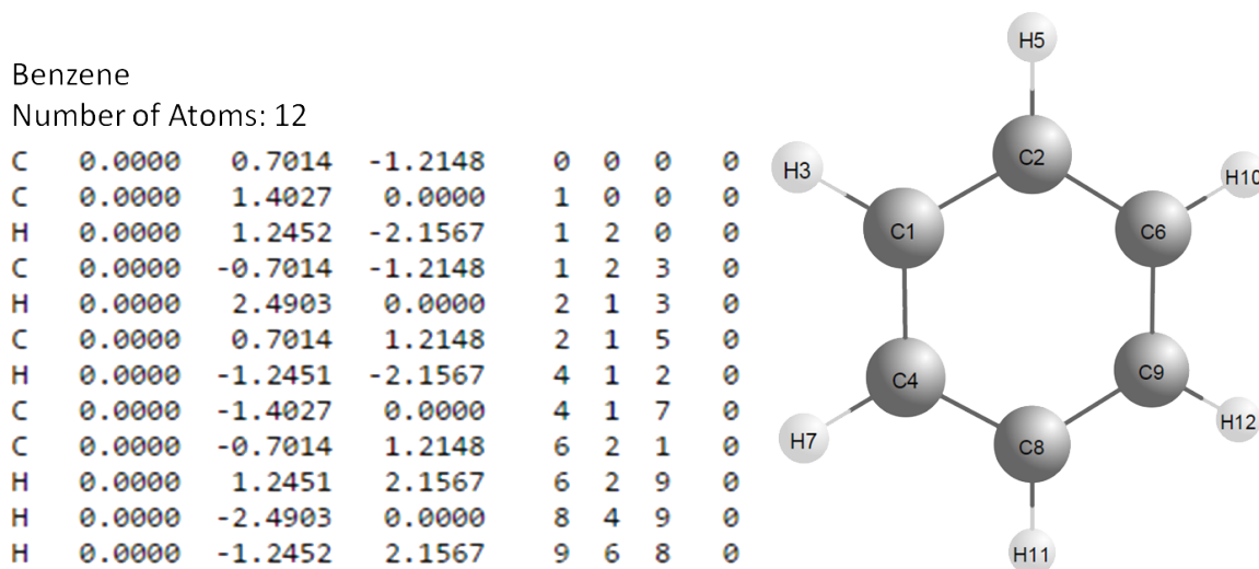
Fig. 5.9.1: Sample of MOL_FILE file and illustration of the corresponding molecular structure.
